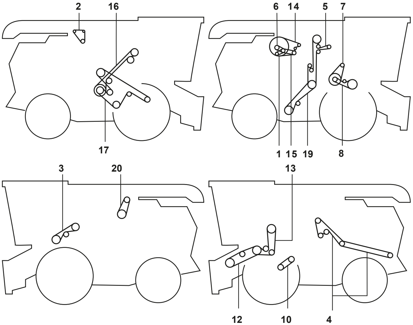
Feederhouse Fixed W/Reverser
