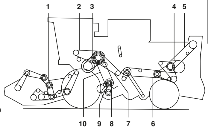
CUTTER PKN1500B
