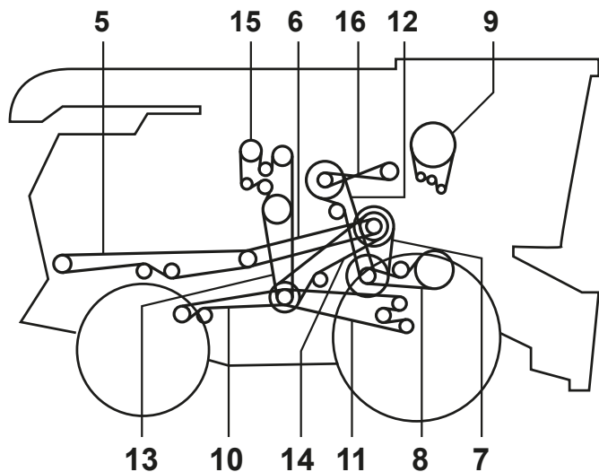
Engine
