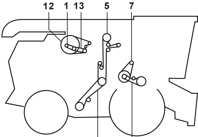
Feederhouse Fixed W/Reverser
