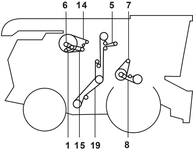
Feederhouse Fixed W/Reverser
