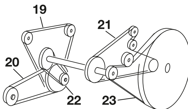
TX 66 (RH)
