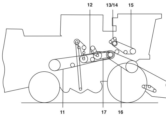
PICK UP PLATFORM
